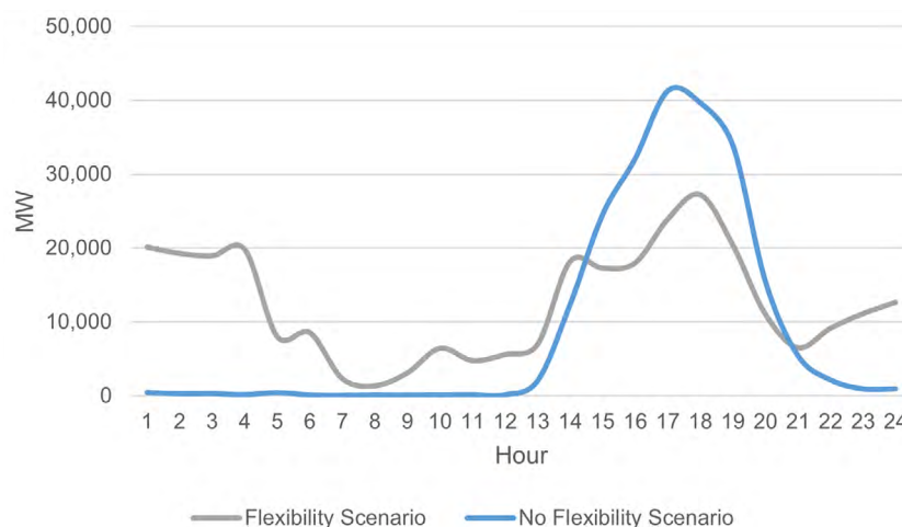
Figure 9: Average daily overall EV charging demand, 2040
