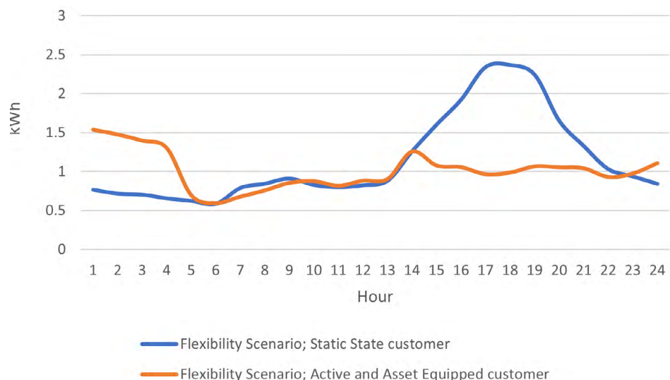
Figure 6: Average daily demand across customer segments, 2030
