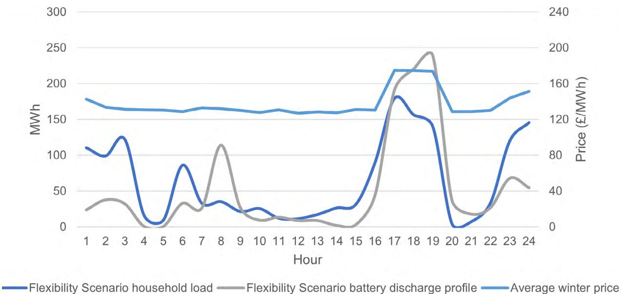
Figure 16: Average daily storage and household demand profile, 2030, overall system level
