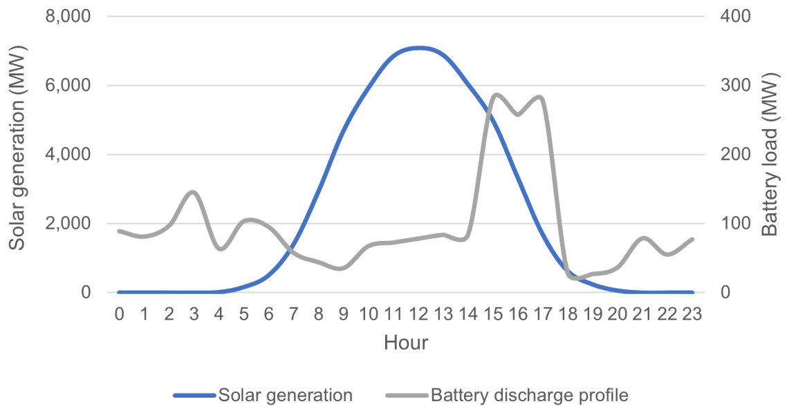
Figure 15: Average solar PV and battery storage daily profile, 2040, all-household level
