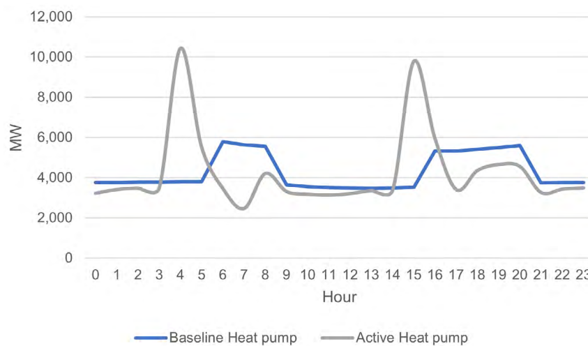
Figure 13: Flexible heat pump consumption during a 24 hour period
