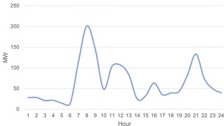
Figure 14: Demand response provided by smart appliances, daily average profile, 2040
