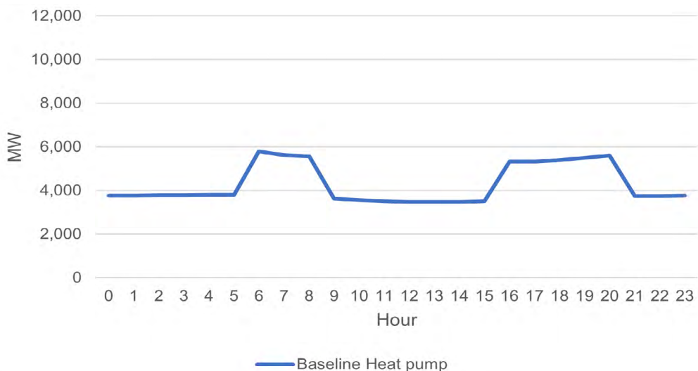
Figure 12: Average total heat pump consumption under a typical demand profile during a 24 hour period
